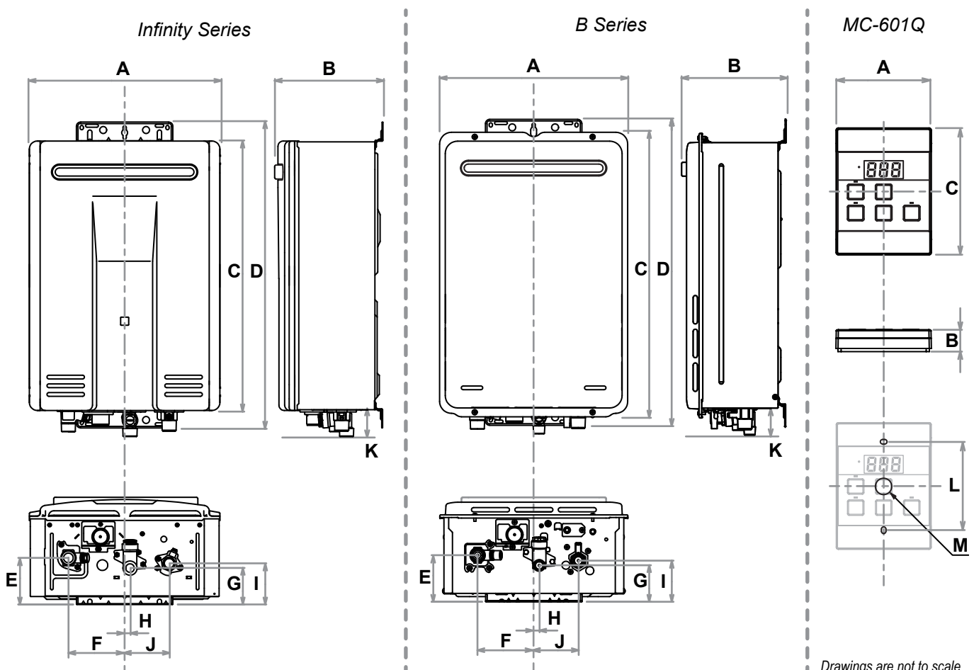
DIAGRAM 1. DIMENSIONS
